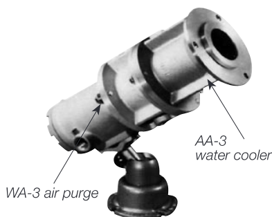
Air purge, water cooling and swivel base mounting accessories
