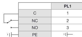
Wiring and connection diagram
